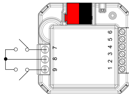
Connection loads to be controlled (relais 5 A)
