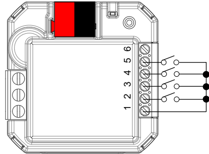
Connection of free-potential contacts
